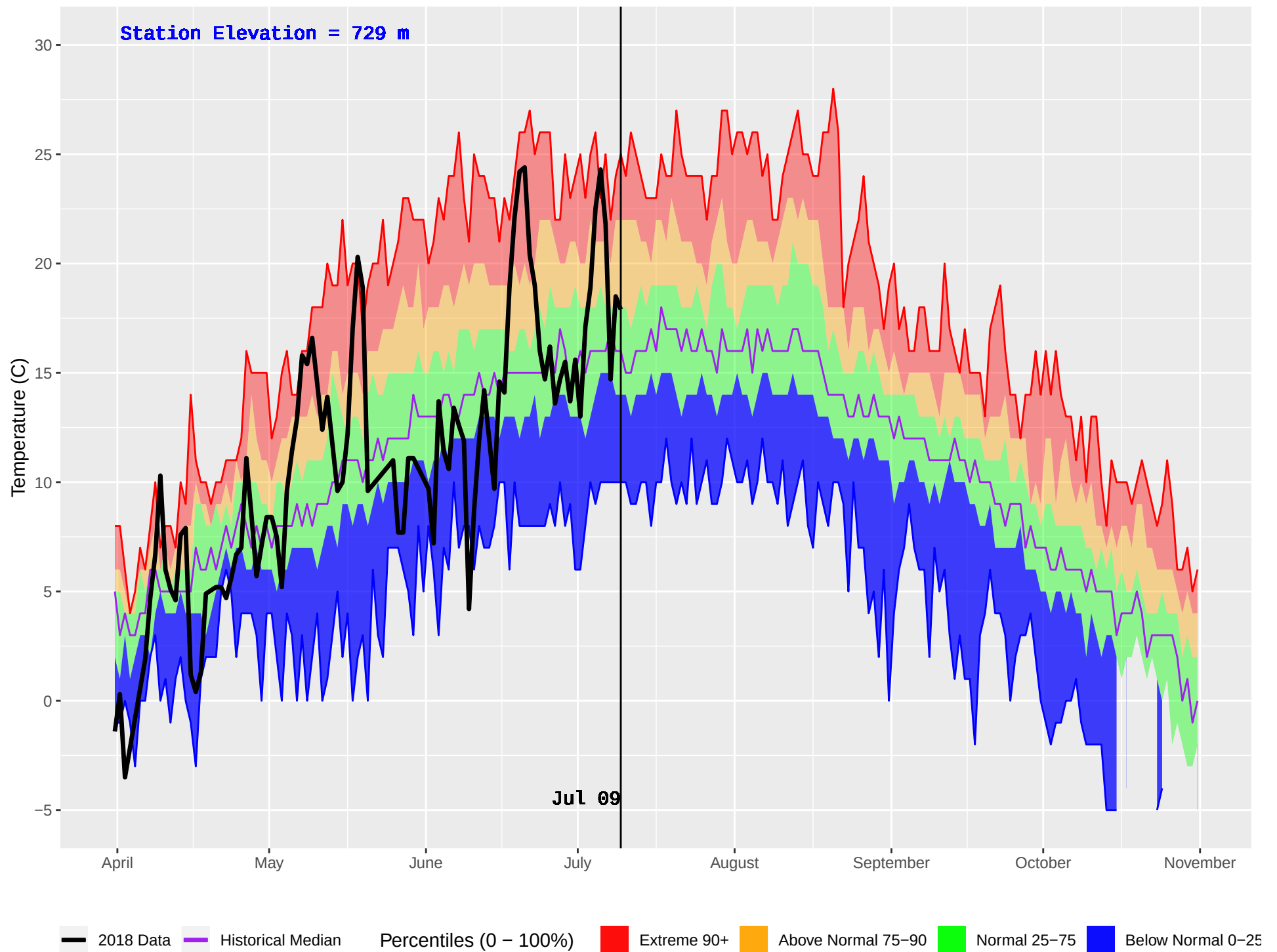
ATLIN (111) : Historical (1977–2016) and Current (2018) Daily Temperature
